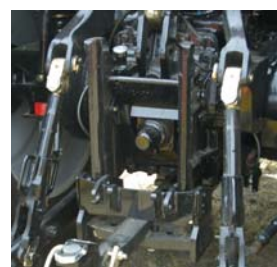
Figure 3: Square masterguard, hinged
